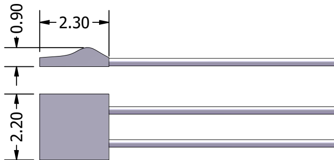
Thin Film Flat Pt100 (TF)
