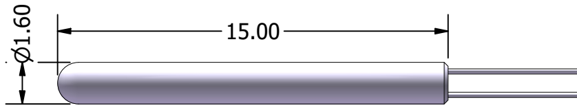
Ceramic Fast Response (FR)
